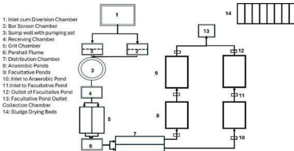
Figure 39 Schematic diagram of WWTP in Birgunj
