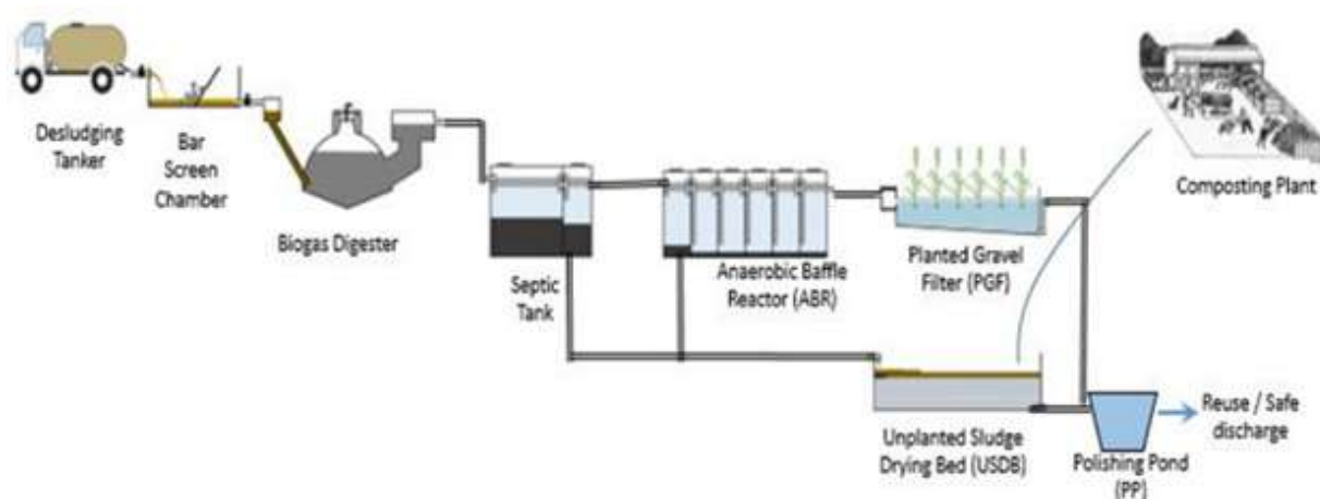
Figure 26 The components and FS flow diagram of Shreekhampur Co-treatment Plant
