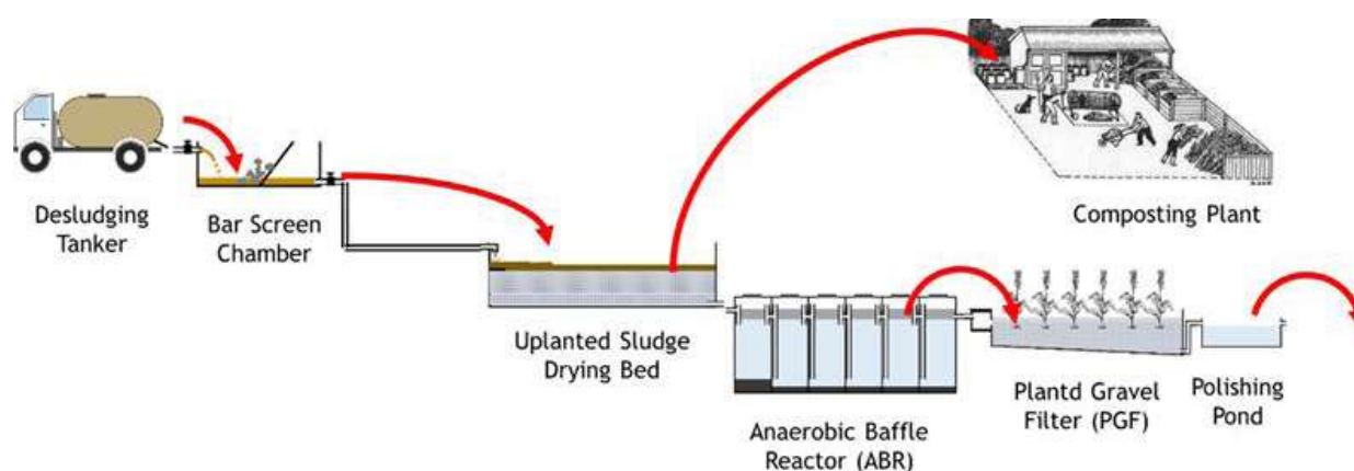
Figure 14 The components and FS flow diagram for Charali FSTP
