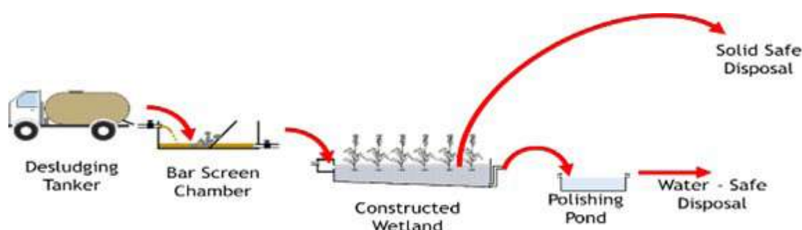
Figure 10 The components and FS flow diagram of Birendranagar FSTP
