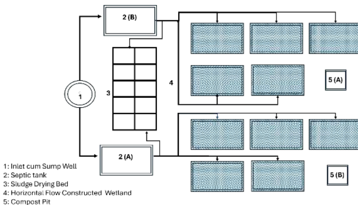
Figure 41 Schematic diagram of WWTP in Ratnanagar Municipality
