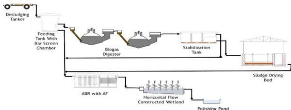
Figure 21 The components and FS flow diagram in Lubhu FSTP
