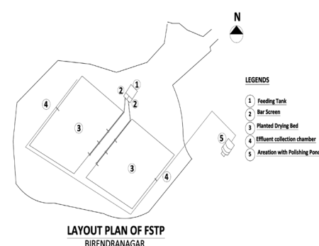
Figure 9 Layout map of Birendranagar FSTP
