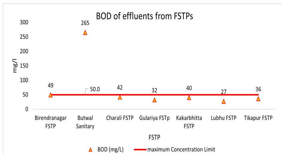
Figure 5: Concentration of BOD in effluent from FSTPs
