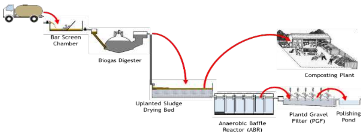
Figure 16 The component and FS flow diagram for Gulariya FSTP
