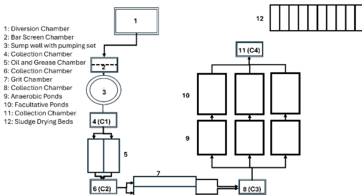
Figure 37 Schematic diagram of the Wastewater treatment plant in Biratnagar
