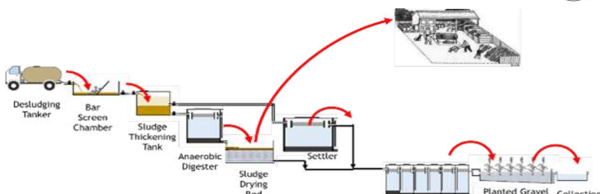
Figure 31 The components and FS flow diagram of Waling FSTP
