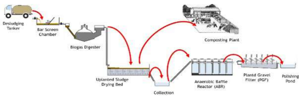
Figure 18 The component and FS flow diagram for Kakarbhitta FSTP
