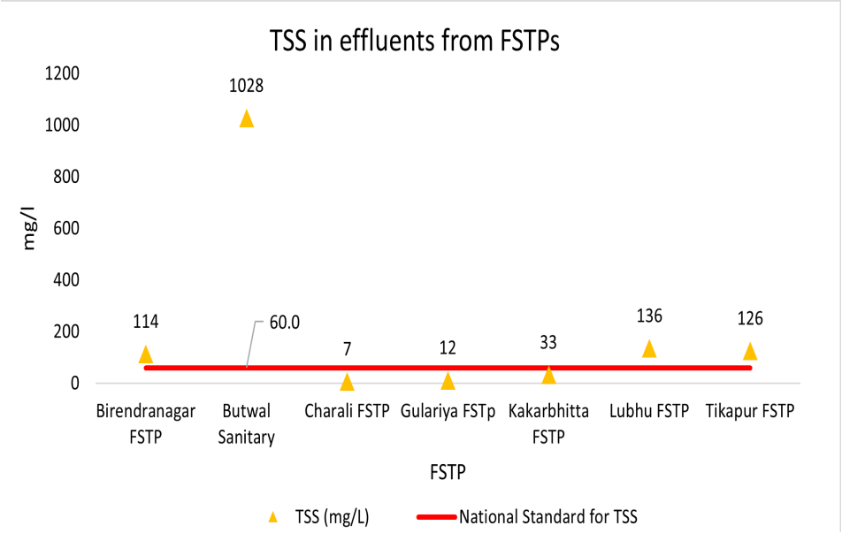
Figure 7 Concentration of TSS in effluents from FSTPs
