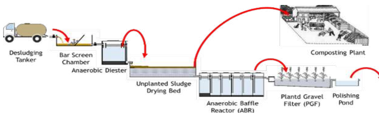
Figure 28 The components and FS flow diagram for Tikapur FSTP
