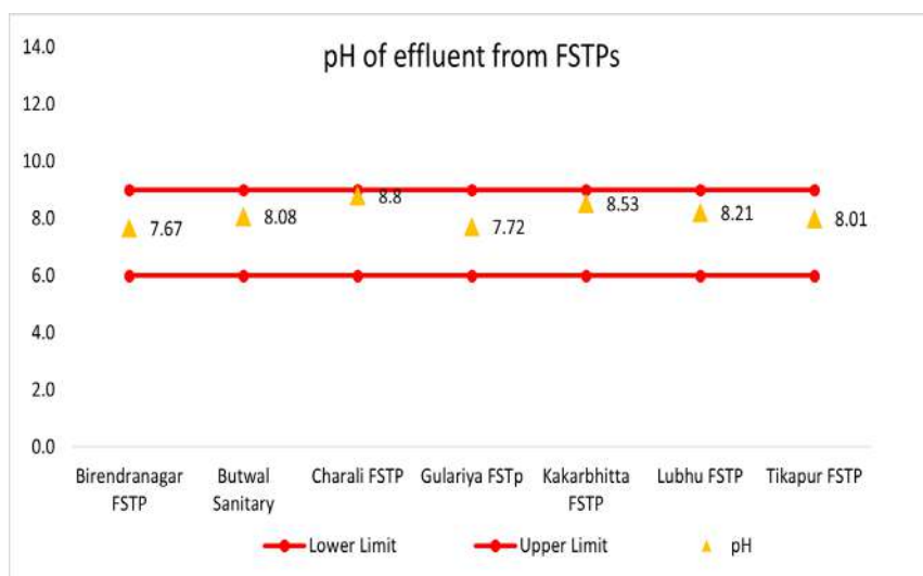
Figure 4: pH values of effluent from FSTPs
