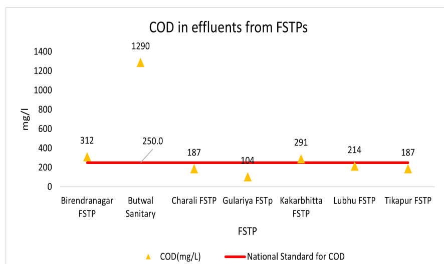
Figure 6 Concentration of COD in effluents from FSTPs
